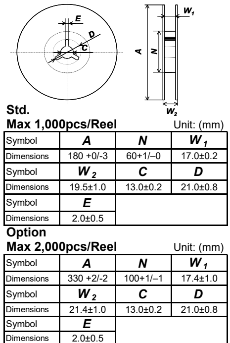
Fig.7 Reel
