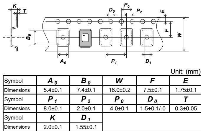
Fig.6 Emboss Carrier Tape
