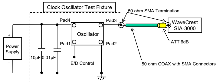
Fig.1 Test Circuits
