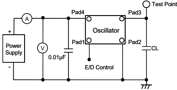
Note: CL includes probe and test fixture capacitance Fig.1 Test Circuits
