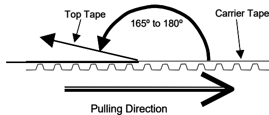
Fig.9 Peeling Strength
