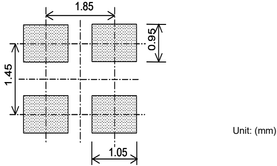
Fig.4 Land pattern
