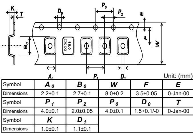
Fig.6 Emboss Carrier Tape
