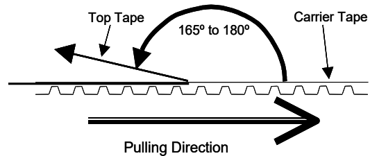
Fig.9 Peeling Strength
