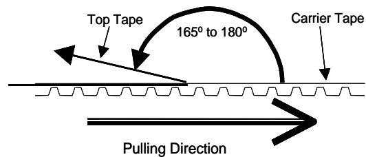
Fig.9 Peeling Strength
