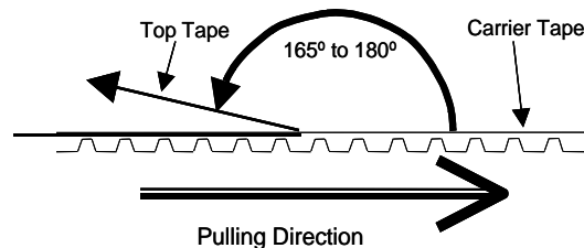
Fig.9 Peeling Strength
