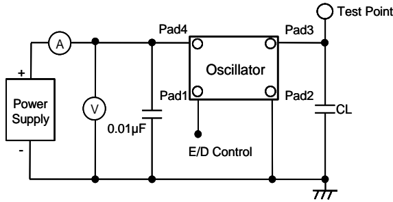
Fig.1 Test Circuits
