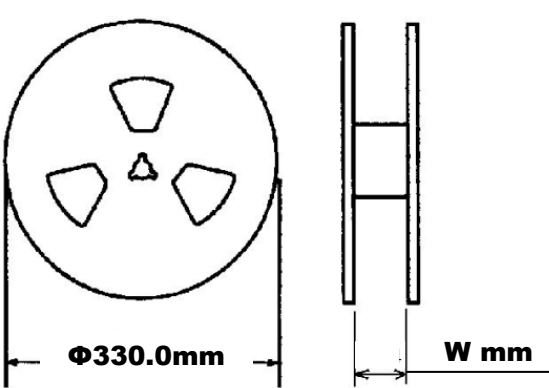
Fig. 3 Emboss tape reel (Plastic)
