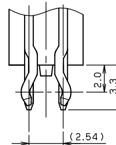
キंक部詳細 (S=5:1) DETAIL OF KINK AREA
