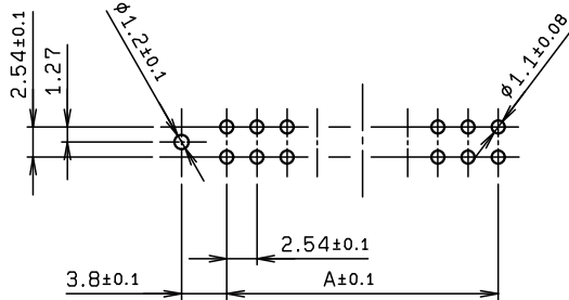
基板穴配列図 MOUNTING LAYOUT
