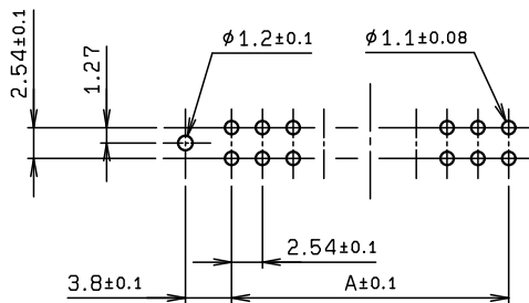
基板穴配図 MOUNTING LAYOUT
