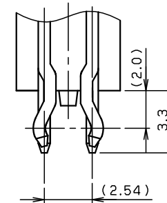
キंक部詳細 (S=5:1) KINKED AREA
