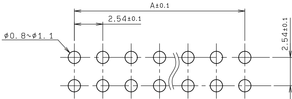
基板穴明け寸法図 MOUNTING LAYOUT
