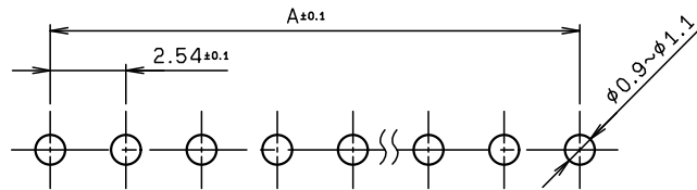
基板穴明寸法図 BOARD HOLE LAYOUT
