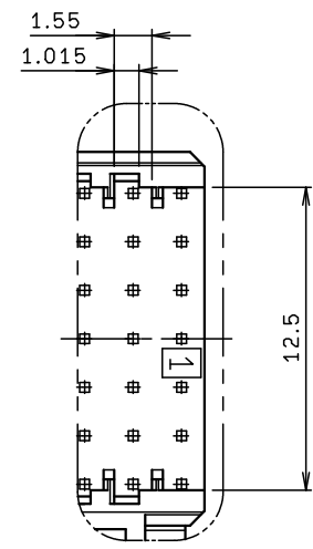
DETAIL-A (S=4/1)
