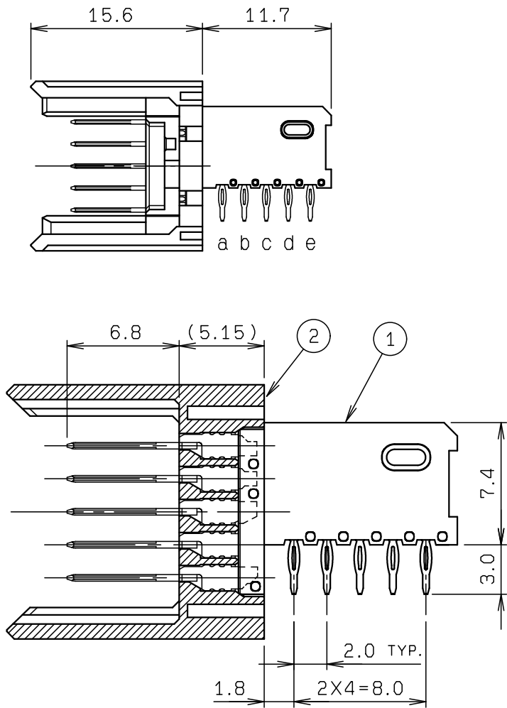
SECT. X-X (S=3:1)
