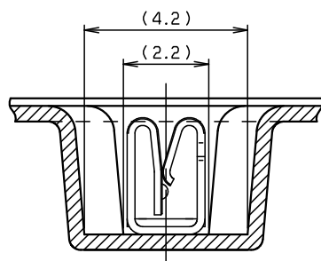
SECT. B-B (S=8:1)
