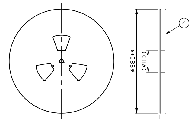
REEL DIMENTION (S=1:6)
