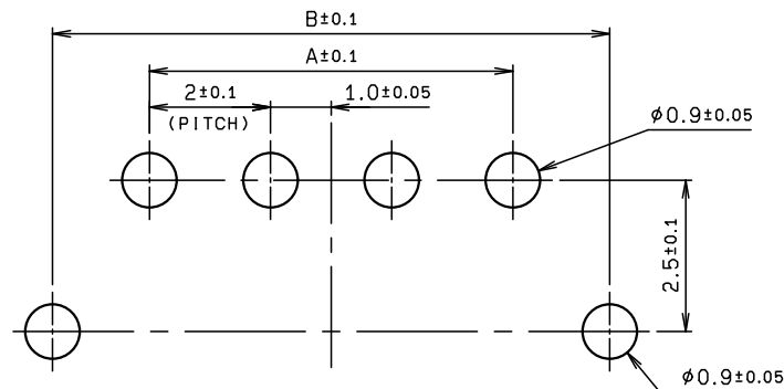
推奨基板寸法 (ドリル穴) RECOMMENDED MOUNTING LAYOUT (DRILL HOLE)
