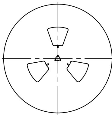
REEL DIMENSION (S=1/5)
