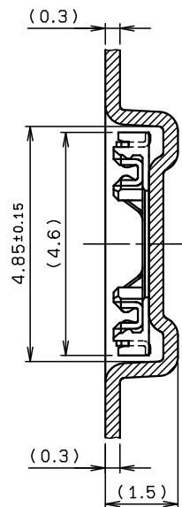
SECT. K-K (S=10/1)
