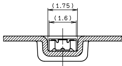
SECT. H-H (S=10/1)
