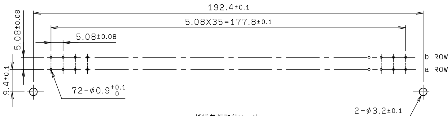
推奨基板取付け寸法 RECOMMENDED BOARD LAYOUT
