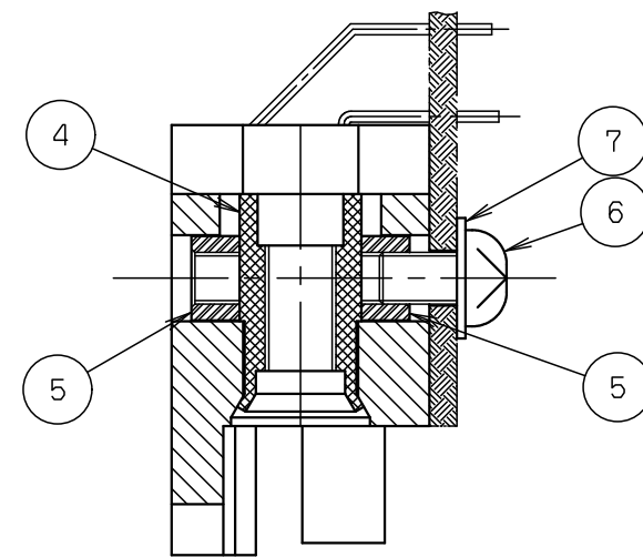
SECT. A-A (S=2:1)
