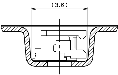
SECT. B-B (S=10/1)
