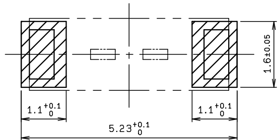
推奨基板寸法 RECOMMENDED P.C BOARD LAYOUT
