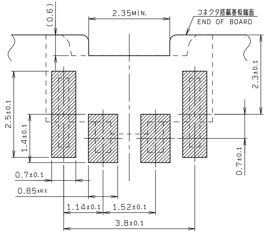
推奨基板寸法 RECOMMENDED P.C BOARD LAYOUT
