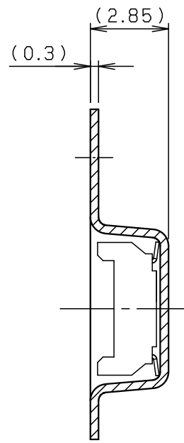
SECT. A-A
