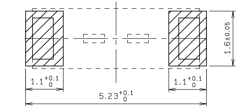
推奨基板寸法 RECOMMENDED P.C BOARD LAYOUT
