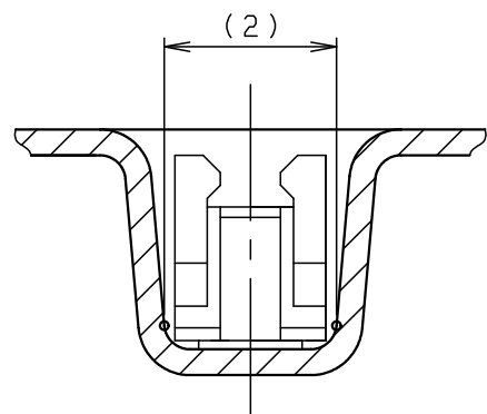
SECT. B-B (S=10:1)
