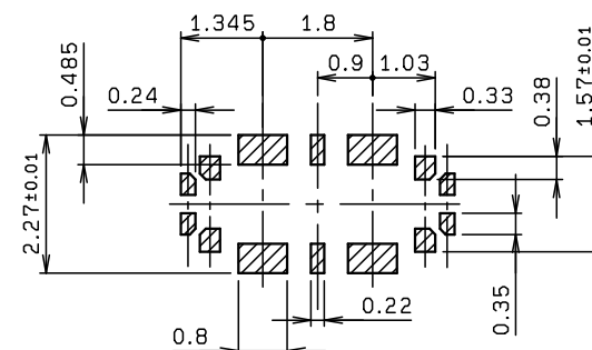
STENCIL LAYOUT
