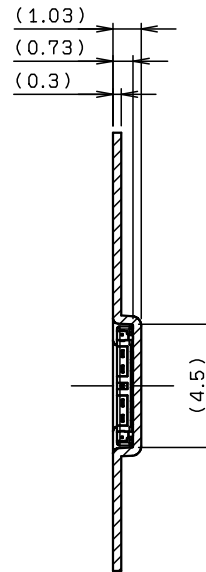
SECT. E-E
