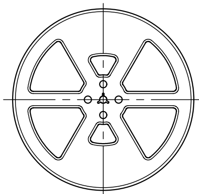
REEL DIMENSION
