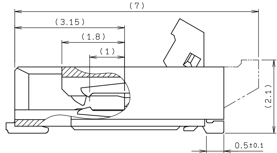
SECT. P-P (S=15:1)
