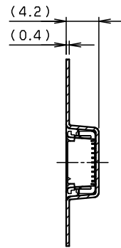
SECT. E-E
