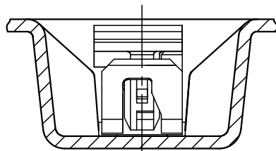
SECT. D-D (S=8:1)
