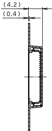
SECT. E-E
