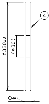
REEL DIMENSION (S=1/5)
