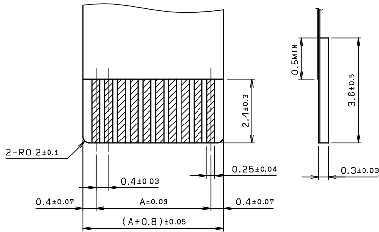
推奨FPC寸法 APPLICABLE FPC
