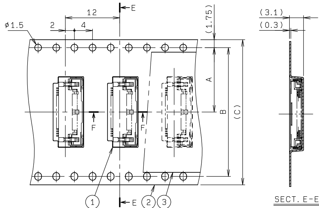
SECT. E-E (~15P)
