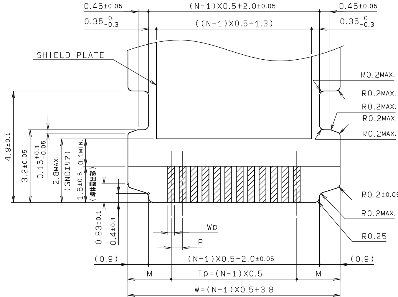
適用FPC/FFC寸法 APPLICABLE FPC/FFC
