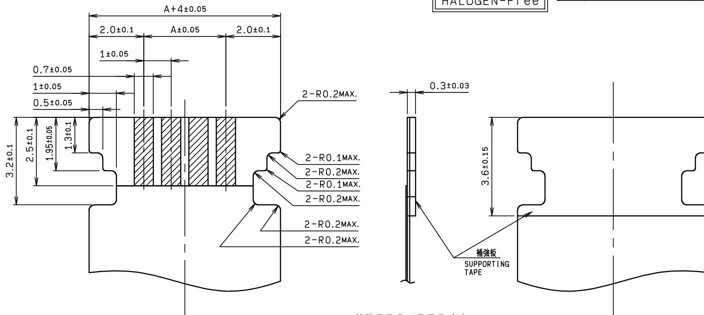
特殊FPC/FFC寸法 DIMENSIONS FOR SPECIAL SHAPED FPC/FFC
