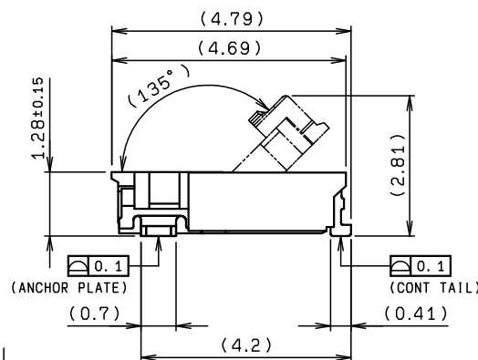
SECT. X-X (S=20:1)
