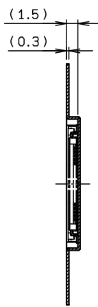
SECT. E-E (9~15P)
