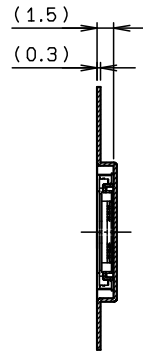
SECT. E-E (4~8P)
