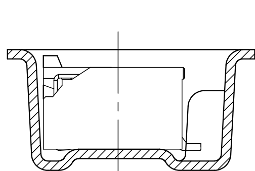
SECT. F-F (S=6:1)
