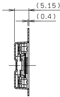
SECT. E-E (~10P) (5.15) (0.4)
