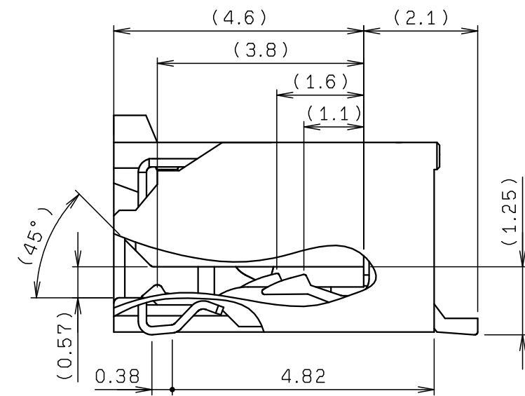
SECT. P-P
