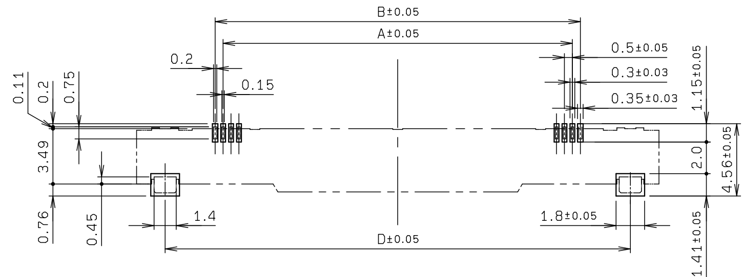
MOUNTING LAYOUT
