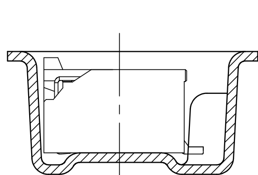
SECT. F-F
