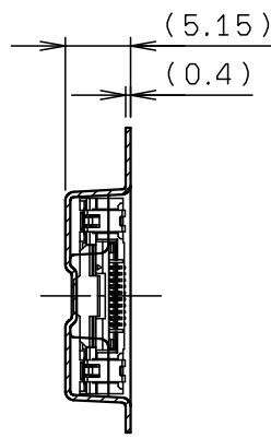
SECT. E-E
