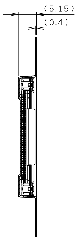
SECT. E-E
