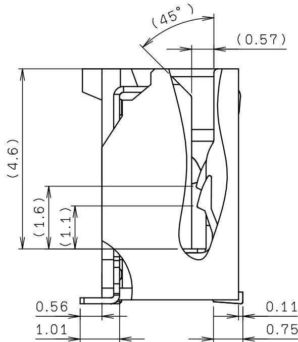
SECT. P-P
