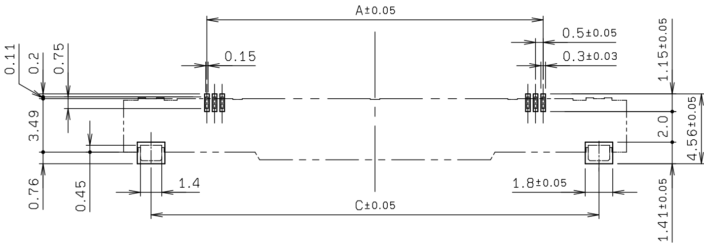
MOUNTING LAYOUT
