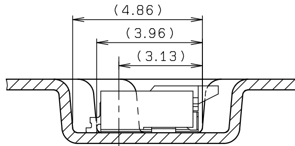
SECT. F-F
