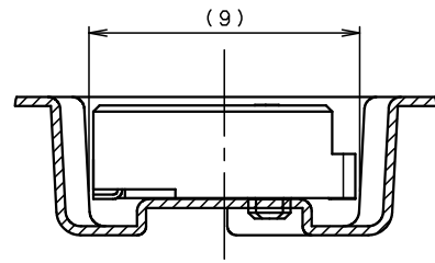
SECT. E-E (S=5/1)
