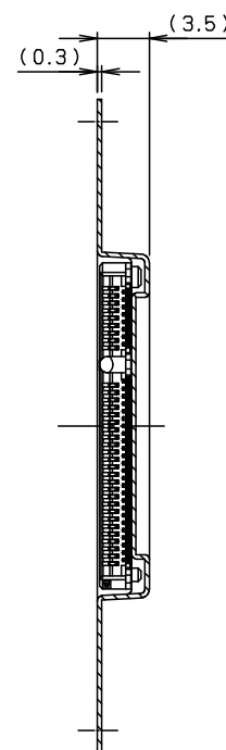
SECT. F-F
