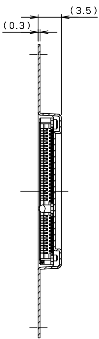
SECT. F-F
