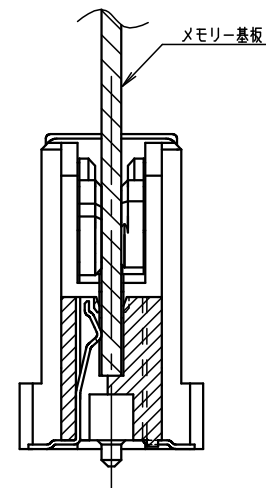
基板挿入状態 FORM OF MOUNTING BOARD
