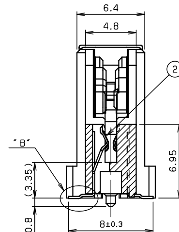
SECT. A-A (S=4/1)
