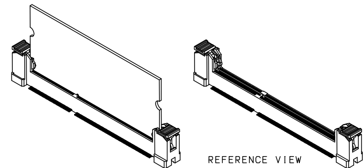
DETAIL "B" (S=15/1)
