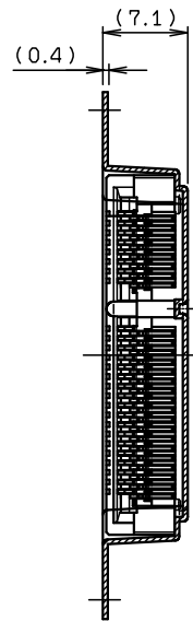
SECT. F-F
