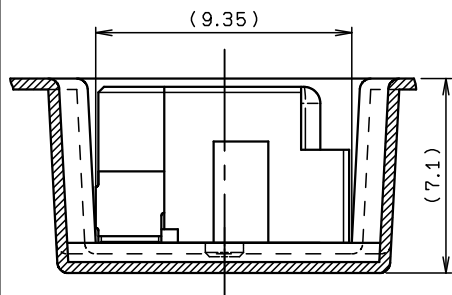
SECT. E-E (S=5:1)
