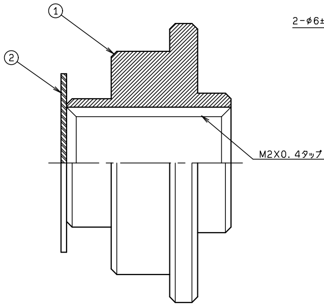
SECT. A-A (S=20:1)
