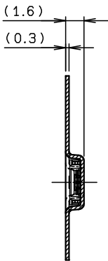
SECT. F-F
