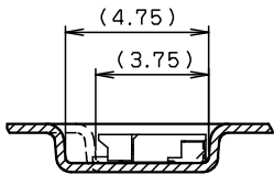
SECT. E-E (s=1/5)
