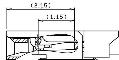
SECT. X-X
