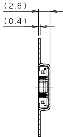
SECT. E-E (5~21P)
