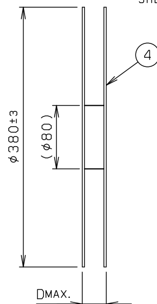
SECT. E-E (22~60P)
