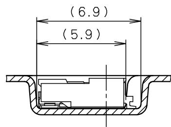
SECT. F-F (S=4:1)
