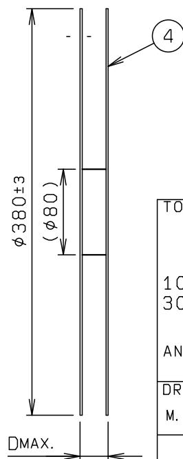
REEL DIMENSION (S=1:5)
