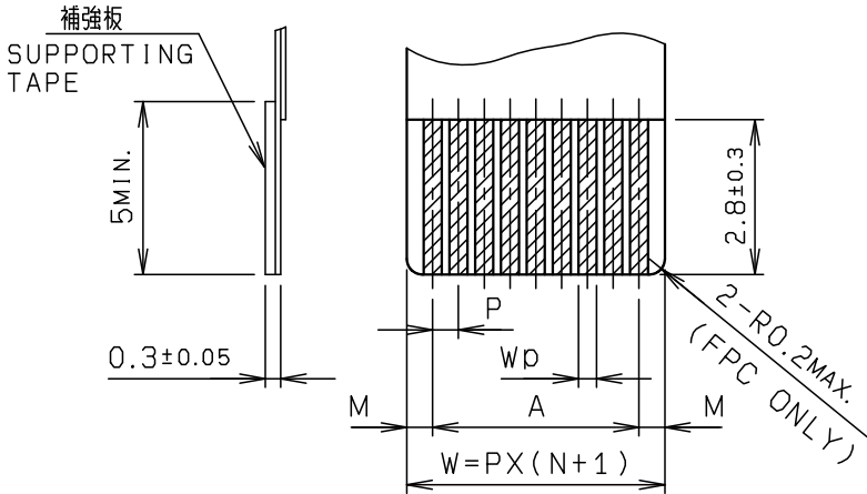
適用FPC/FFC寸法 APPLICABLE FPC/FFC
