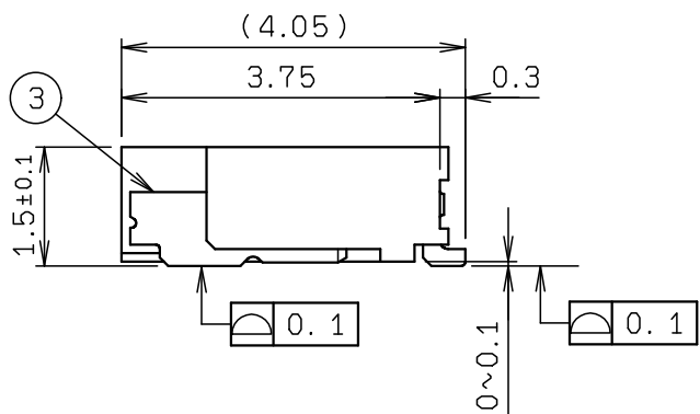
SECT. D-D (S=20:1)
