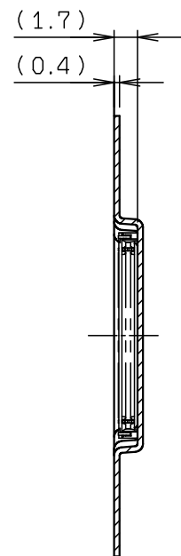
SECT. E-E (25P~)
