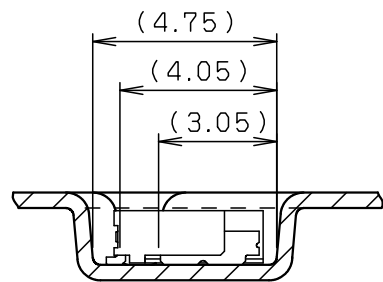
SECT. F-F (S=5:1)
