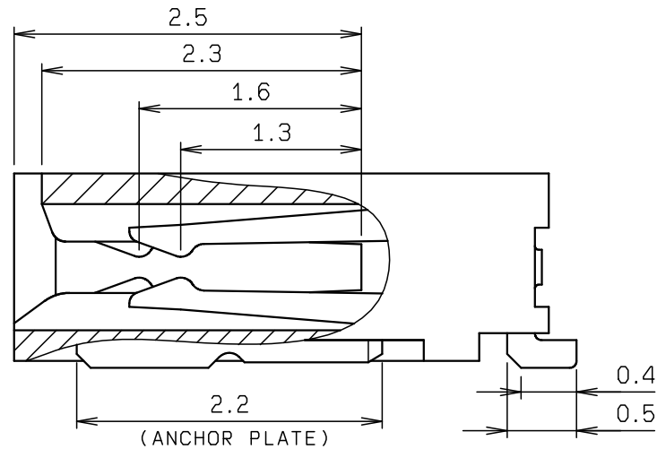
SECT. D-D (S=20:1)
