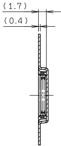
SECT. E-E (~24P)
