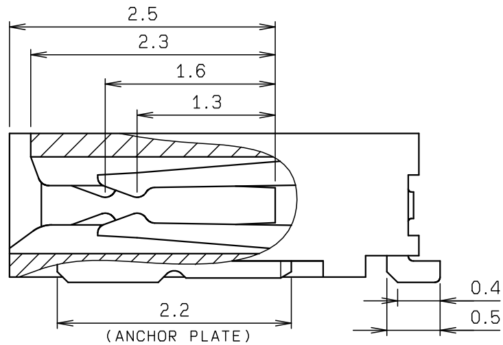
SECT. D-D (S=20:1)
