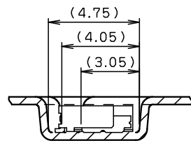
SECT. F-F (S=5:1)
