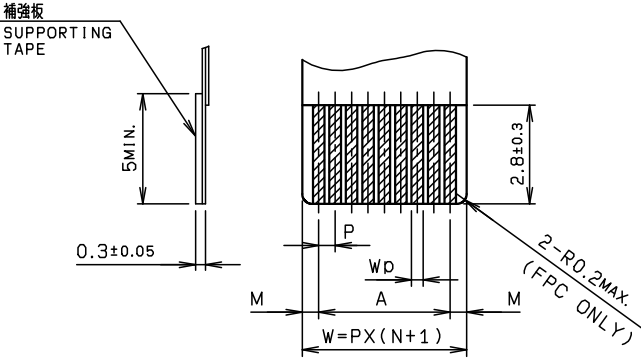
適用FPC/FFC寸法 APPLICABLE FPC/FFC
