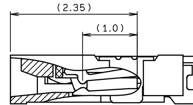
SECT. X-X
