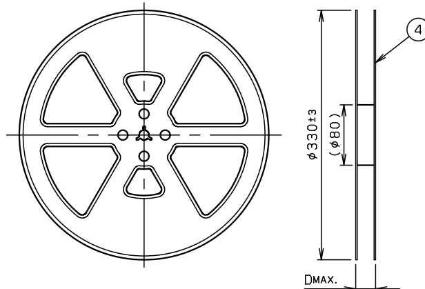
REEL DIMENSION (S=1:5)
