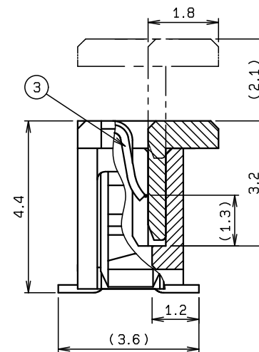
SECT. X-X
