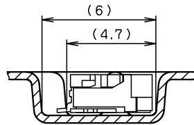
SECT. E-E (S=5:1)
