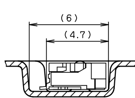
SECT. E-E (S=5:1)
