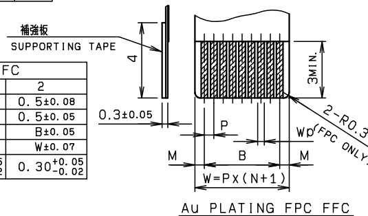
適用FPC FFC寸法 APPLICABLE FPC FFC
